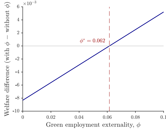
Figure 6: Welfare gains as a function of the externality parameter \phi ( \phi^* \approx 0.062 ).
