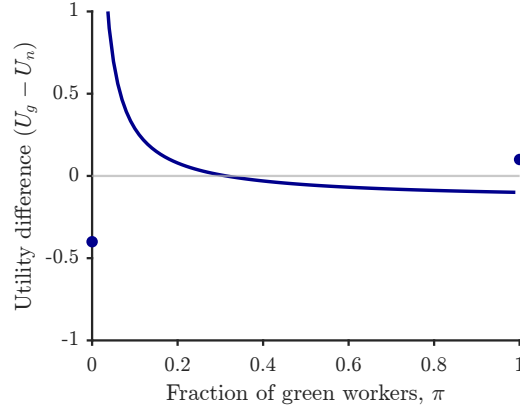
Figure 1: Multiple Equilibria
